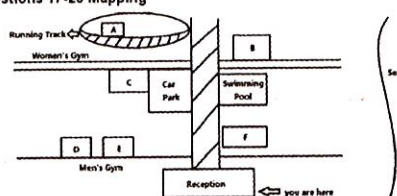
Questions 17-20 Mapping
